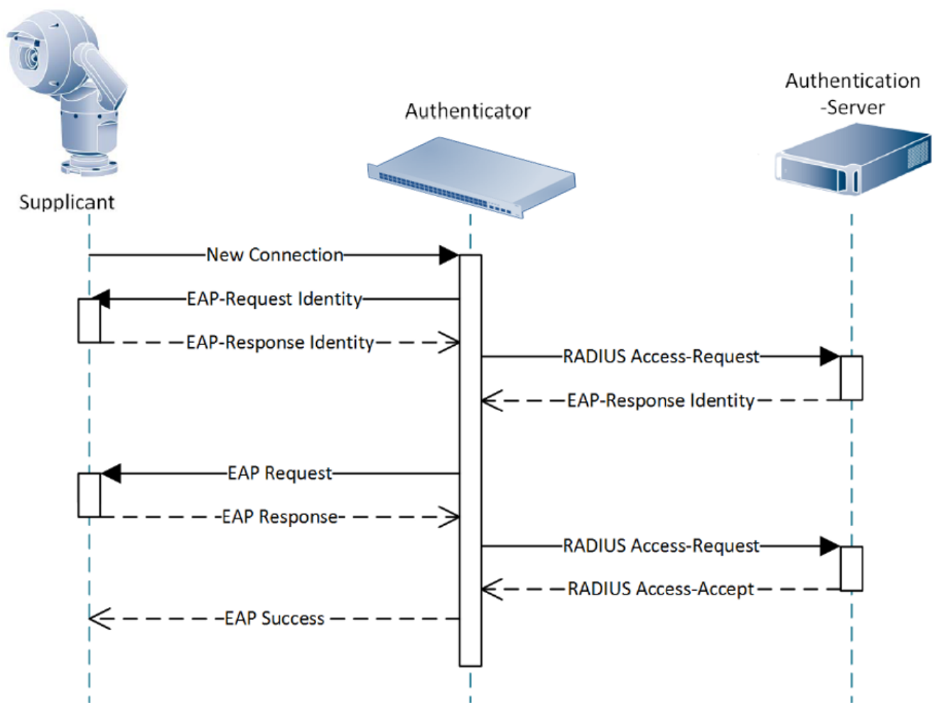
Figure 2: 802.1x Authentication Sequence Diagram
