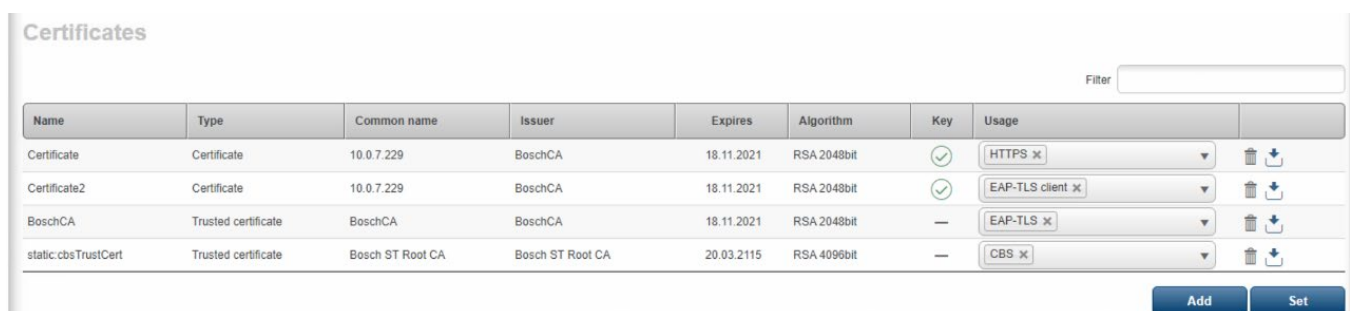
Figure 4: Example EAP/TLS certificates stored in a Bosch camera (FW6.40 and higher)
