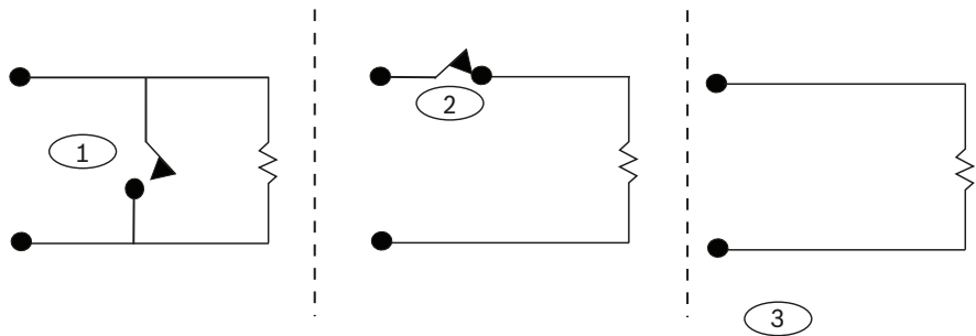
Figure 16.1: Single EOL resistor option
