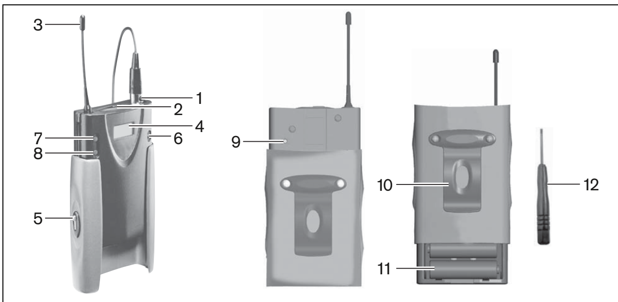
figure 3.7: Belt-pack transmitter
