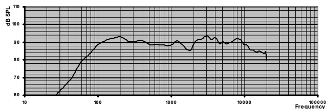
Frequenzgang
