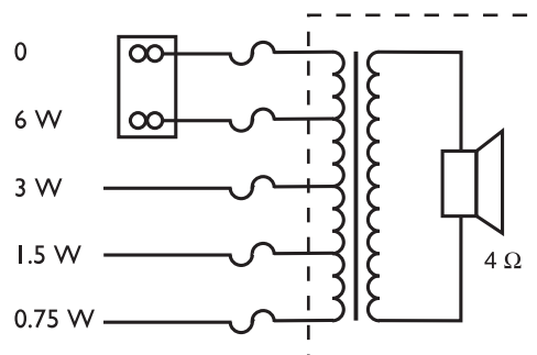
Schema circuitale
