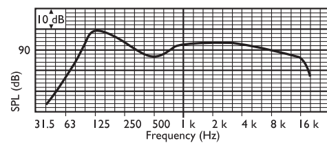
Fig. 10: Frequency response
