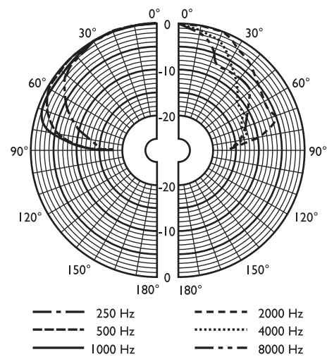
Fig. 11: Polar diagram
