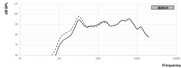
Frequency response
