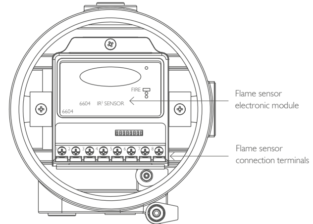
Figure 2. Enclosure with front cover removed
