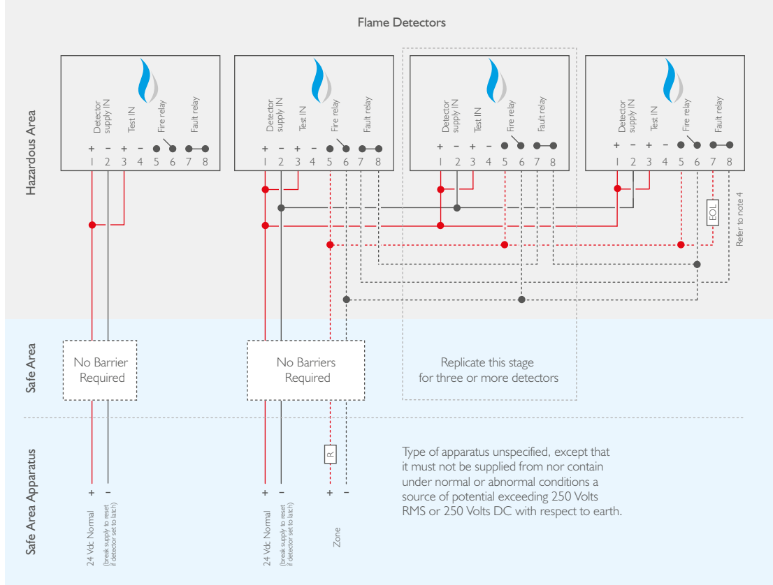
Figure 3. Ex d system connection diagram
