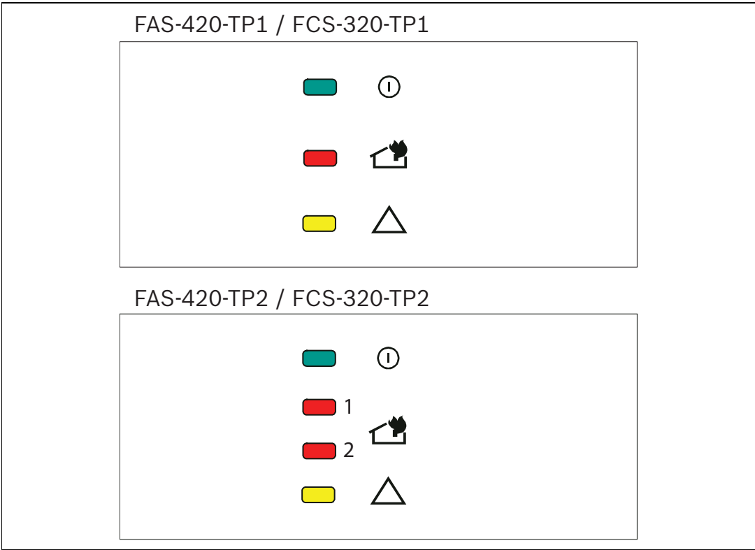
图 2.8 FCS-320-TP1/FCS-320-TP2 显示
